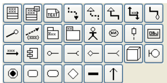
Figure 6.10: UML
