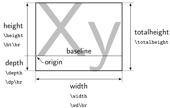
Figure 1: Box dimensions. Shown are also the \LaTeX macros and the \TeX primitives. Here \backslash br stands for a box register. Note that the depth is a positive values on its own downwards pointed axes.
